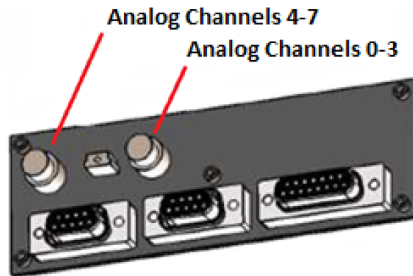
Figure 52: Analog Channel Connectors
