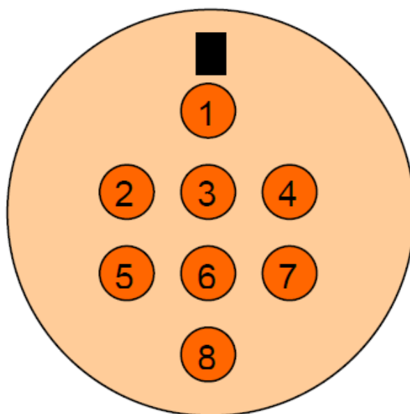
Figure 53: Analog Pin Map
